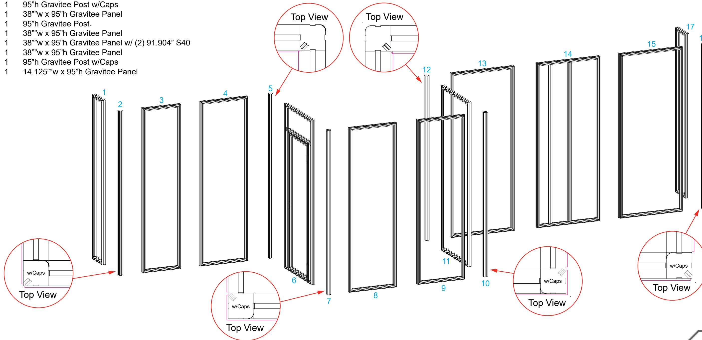
Completed Assembly
